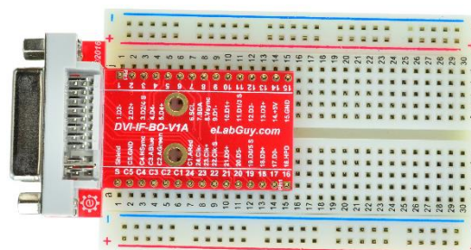
Figure 2: Example of connecting the DVI-IF-BO-V1A on a breadboard
